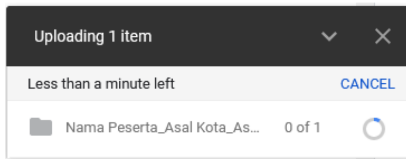
Gambar 7 proses upload
