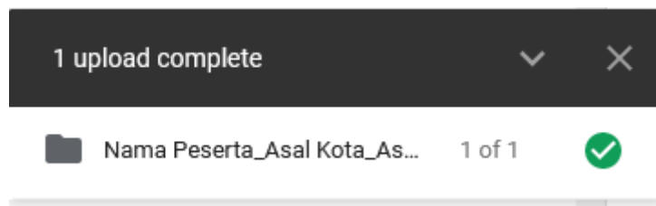
Gambar 8 selesai upload
