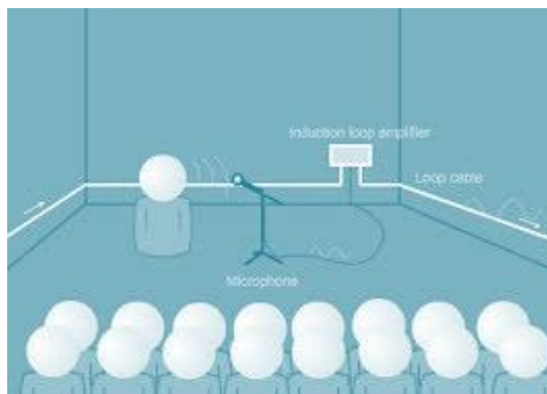
Gambar 3. 1 Sistem Induction Loop
