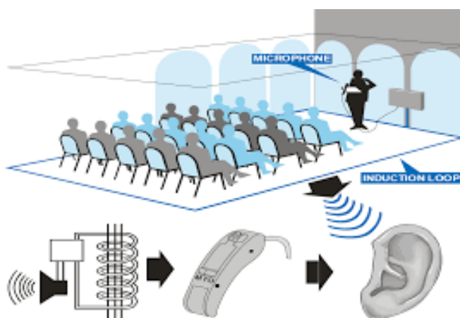
Gambar 3. 1 Sistem Induction Loop
