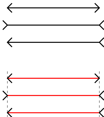
Gambar 7.1: Garis Müller-Lyer
