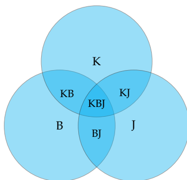
Gambar 1.1: Analisis tradisional
